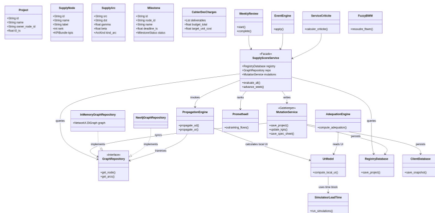
Figure 10: System architecture: single facade, audited writes, per-node persistence
