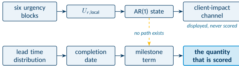
Figure 17: Inside the forecast rollout, the autoregressive state fitted to computed urgency feeds only the client-impact channel. The scored quantity depends on a lead-time draw and, on a chain with no exogenous event, on nothing else.
